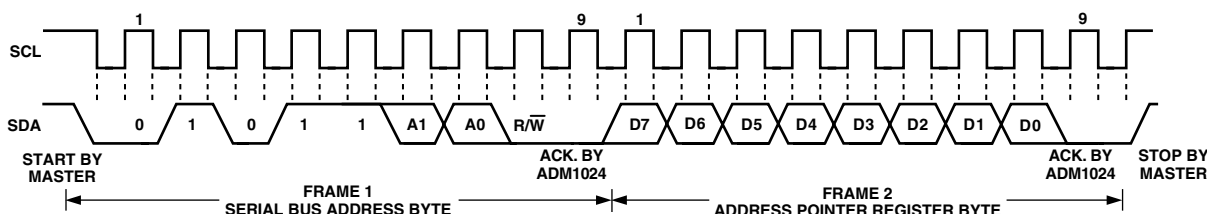
Figure 2b. Writing to the Address Pointer Register Only
