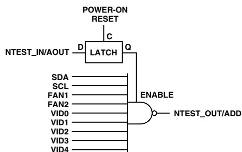
Figure 17. NAND Tree
