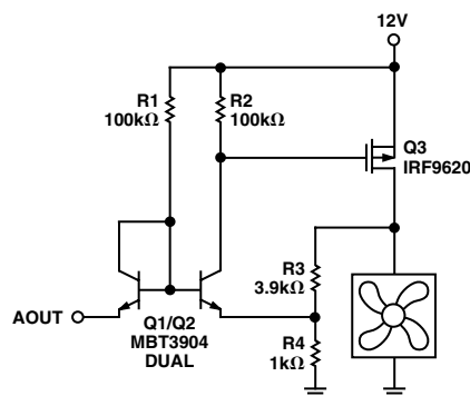
Figure 9d. Discrete Fan Drive Circuit with P-Channel MOSFET, Single Supply
