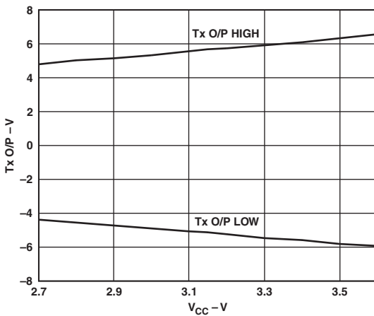
TPC 2. Transmitter Output Voltage vs. V CC
