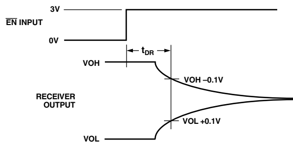
Figure 13. Receiver-Disable Timing
