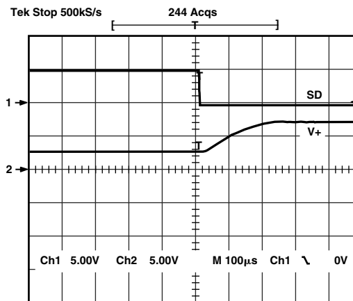
Figure 14. Charge Pump V+ Exiting Shutdown
