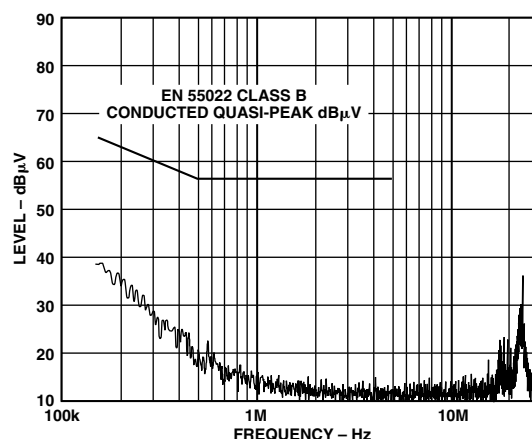
Figure 29. Conducted Emissions Plot
