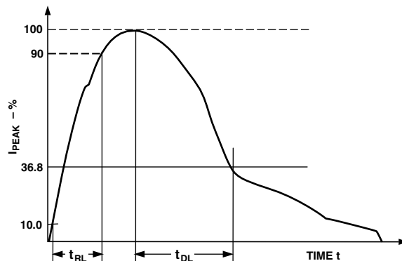
Figure 23. Human Body Model ESD Current Waveform
