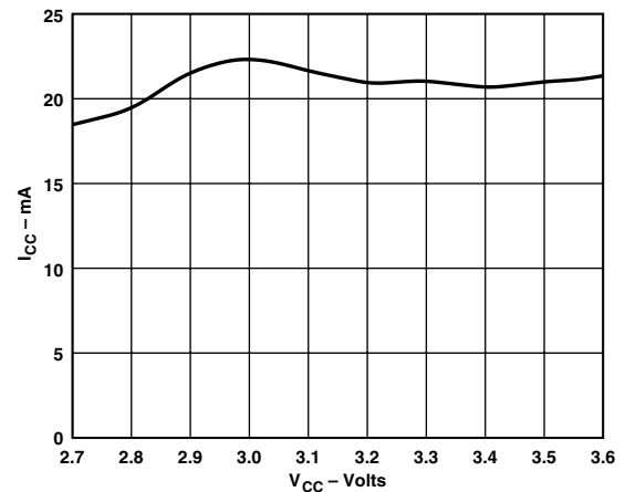
Figure 6. Power Supply Current vs. Power Supply Voltage (R L = 3 k \Omega )
