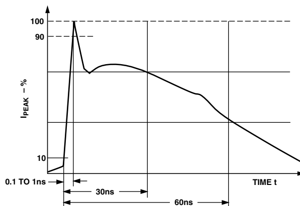
Figure 24. IEC1000-4-2 ESD Current Waveform
