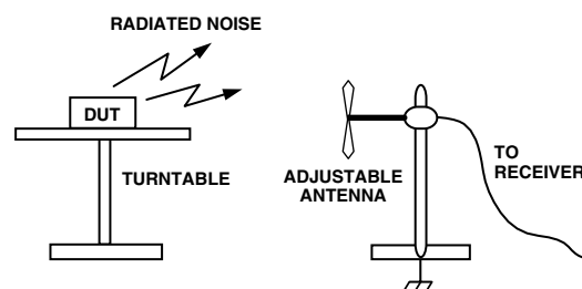
Figure 30. Radiated Emissions Test Setup
