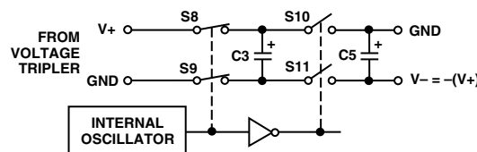
Figure 16. Charge Pump Voltage Inverter
