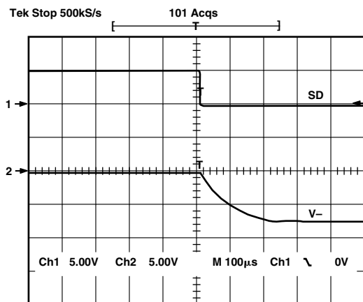
Figure 13. Charge Pump V- Exiting Shutdown
