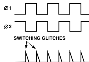
Figure 28. Switching Glitches
