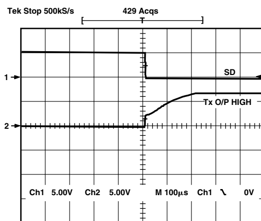
Figure 11. Transmitter Output (High) Exiting Shutdown
