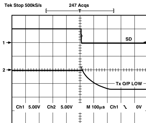
Figure 12. Transmitter Output (Low) Exiting Shutdown
