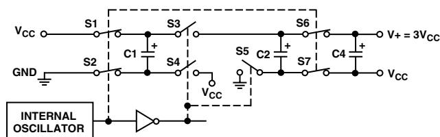
Figure 15. Charge Pump Voltage Tripler
