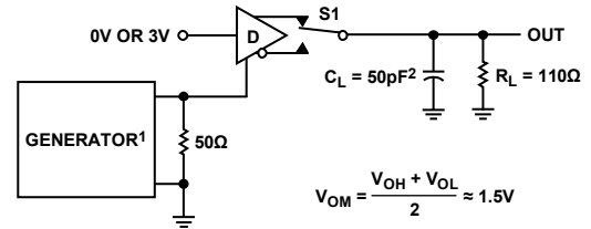
Figure 11. Driver Propagation Delays
