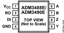
Figure 5. ADM3488E/ADM3490E Pin Configuration
