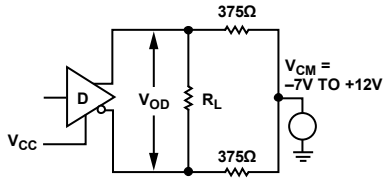
Figure 8. Driver Differential Output Voltage with Varying Common-Mode Voltage
