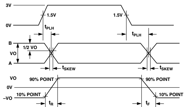
Figure 9. Driver Propagation Delay, Rise/Fall Timing
