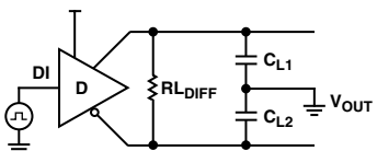
Figure 3. Driver Differential Output Delay Test Circuit
