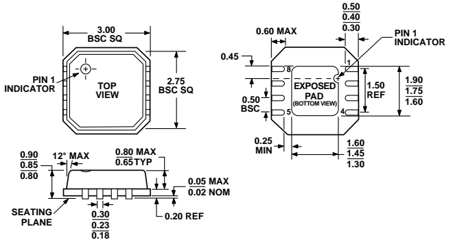
Figure 29. 8-Lead Lead Frame Chip Scale Package [LFCSPP] (CP-8-2) Dimensions shown in millimeters
