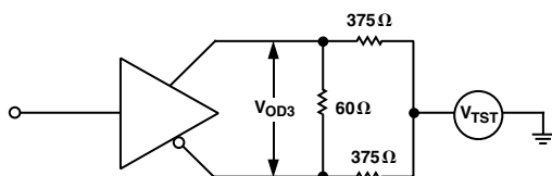
Figure 2. Driver Enable/Disable Test Circuit
