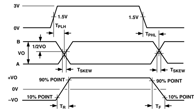
Figure 6. Driver Propagation Delay, Rise/Fall Timing
