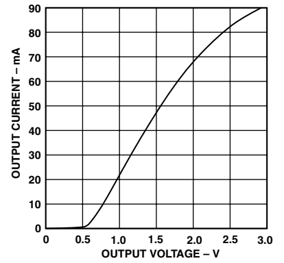
TPC 3. Driver Output Low Voltage vs. Output Current
