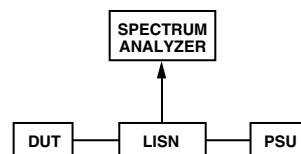
Figure 14. Conducted Emissions Test Setup
