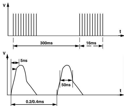
Figure 11. IEC1000-4-4 Fast Transient Waveform
