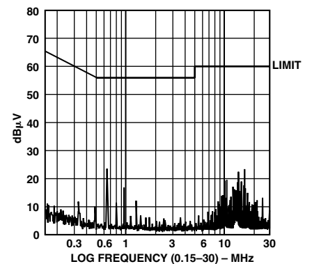
TPC 9. Conducted Emissions
