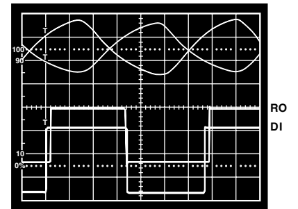
TPC 6. Driving 4000 ft. of Cable
