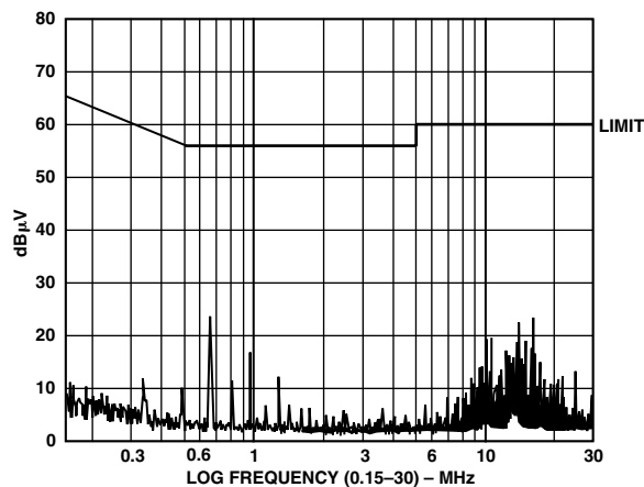
Figure 15. Conducted Emissions
