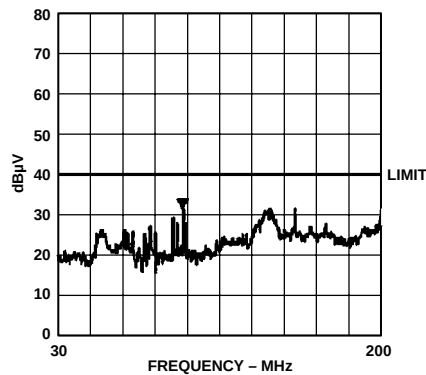
Figure 17. Radiated Emissions
