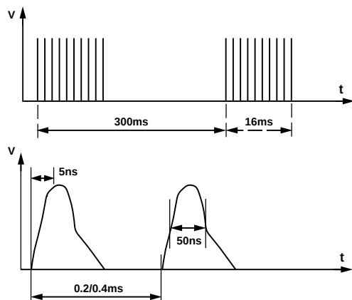
Figure 20. IEC1000-4-4 Fast Transient Waveform
