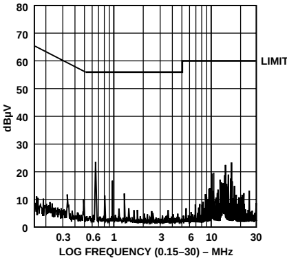
Figure 24. Conducted Emissions
