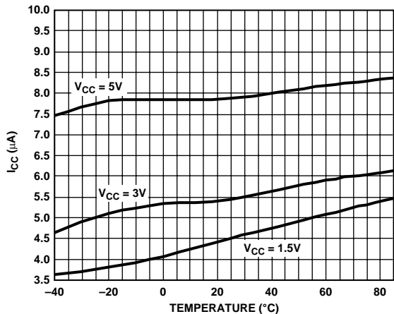
Figure 6. Supply Current vs. Temperature (ADM6316/ADM6317/ADM6318/ADM6320/ADM6321)
