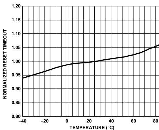
Figure 11. Normalized Reset Timeout Period vs. Temperature
