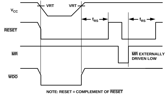
Figure 3. \overline{\text{RESET}} , MR and WDO Timing
