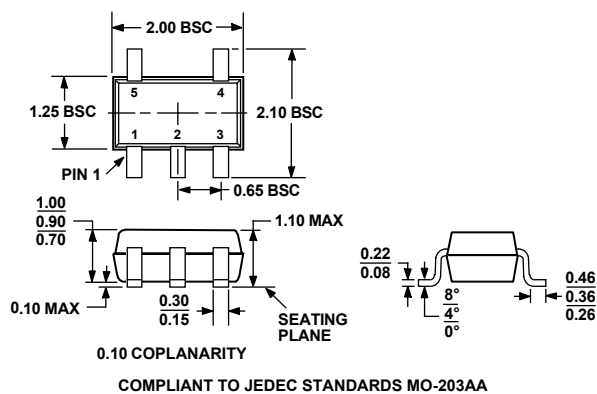
Figure 15. 5-Lead Plastic Surface-Mount Package [SC-70] (KS-5)
