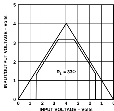
Figure 9. Power-Up/Power-Down on ADP3302AR3. \overline{SD} = 3V or V_{IN}
