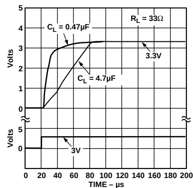
Figure 16. Turn On ADP3302AR3
