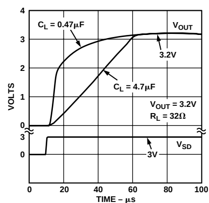
Figure 16. Turn On
