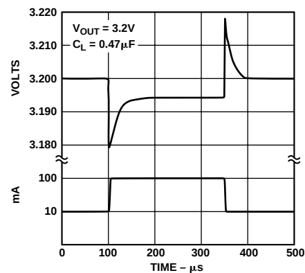
Figure 13. Load Transient
