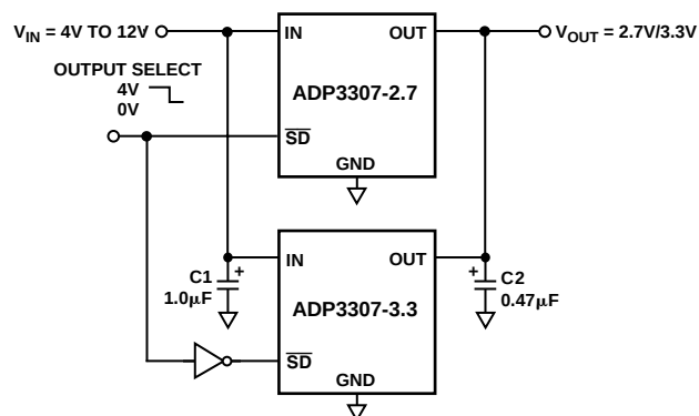
Figure 22. Crossover Switch
