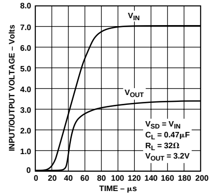
Figure 10. Power-Up Overshoot
