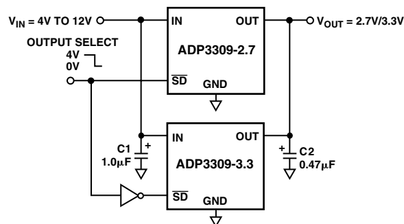
Figure 3. Crossover Switch
