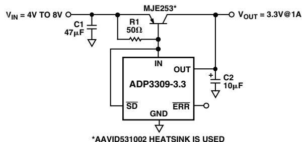
Figure 4. Higher Output Current Linear Regulator
