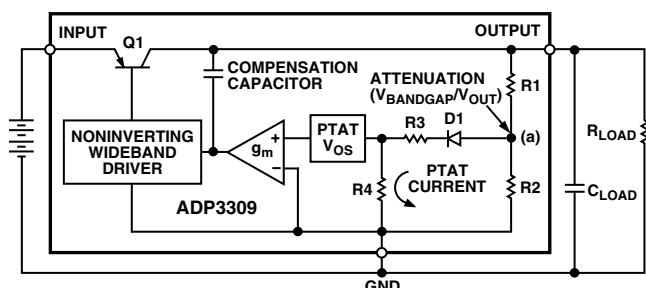
Figure 2. Functional Block Diagram
