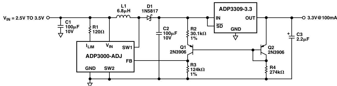
Figure 5. Constant Dropout Post Regulator
