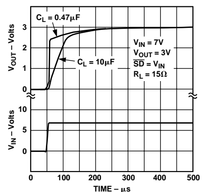
Figure 10. Power-Up Response
