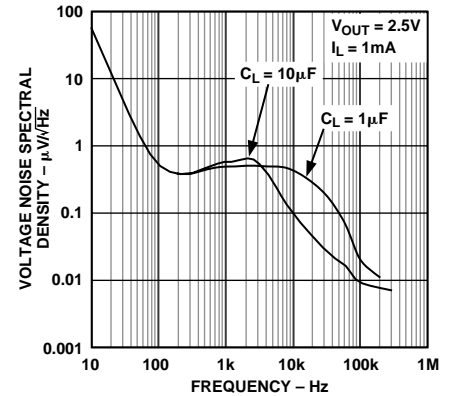
TPC 18. Output Noise Density
