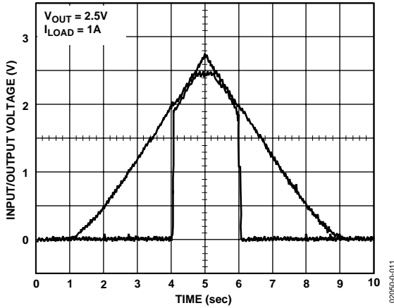
Figure 11. Power-Up/Power-Down
