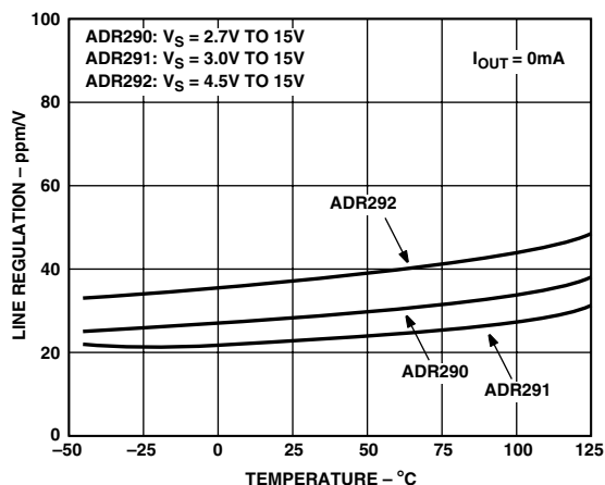
TPC 8. ADR290/ADR291/ADR292 Line Regulation vs. Temperature
