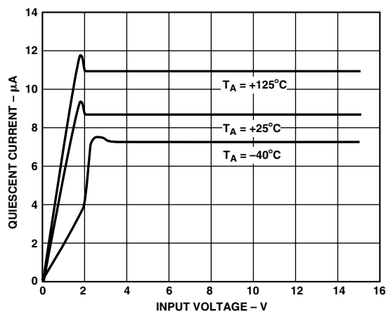
TPC 4. ADR290 Quiescent Current vs. Input Voltage
