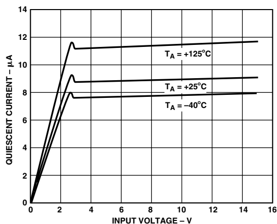
TPC 5. ADR291 Quiescent Current vs. Input Voltage
