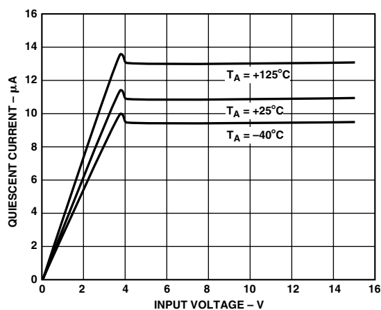
TPC 6. ADR292 Quiescent Current vs. Input Voltage
