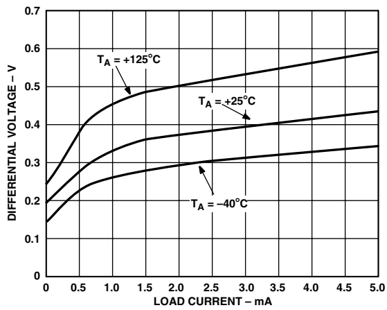
TPC 9. ADR292 Minimum Input-Output Voltage Differential vs. Load Current
