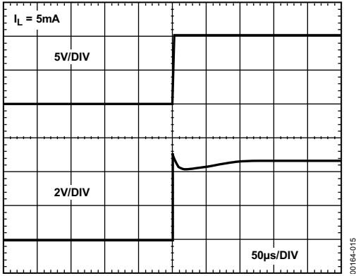
Figure 15. Turn-On Time
