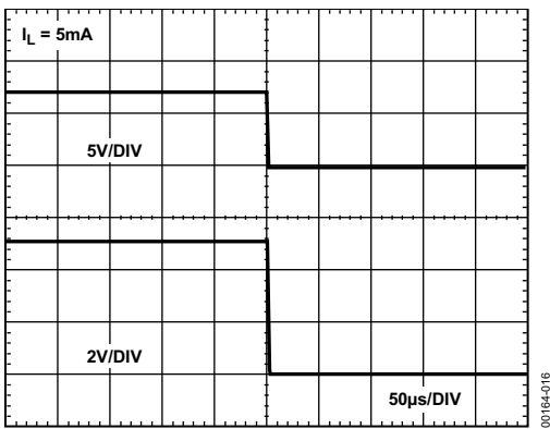
Figure 16. Turn-Off Time
