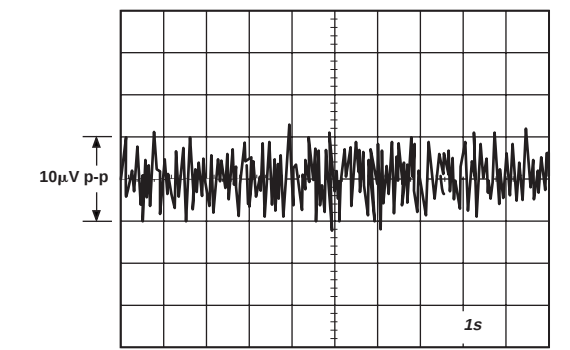
Figure 12. 0.1 Hz to 10 Hz Noise
