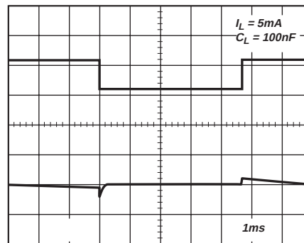
Figure 17. Load Transient
