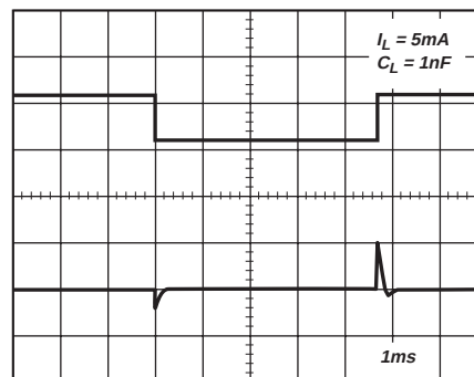
Figure 16. Load Transient
