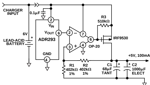
Figure 23. Voltage Regulator for Portable Equipment
