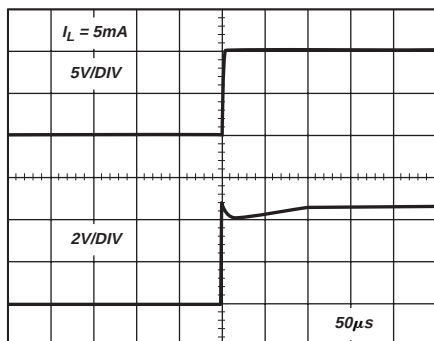
Figure 13. Turn-On Time
