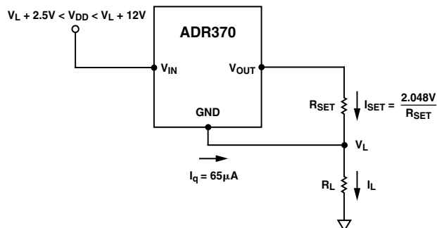
Figure 5. Low Cost Current Source
