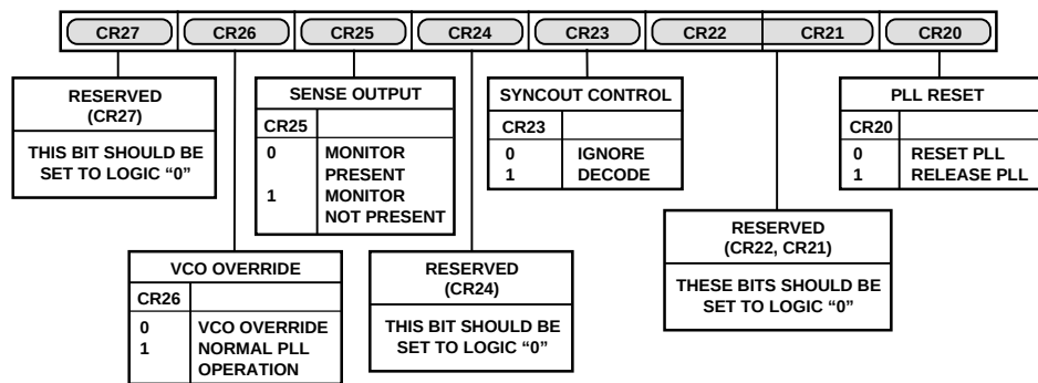
Figure 8. Command Register 2
