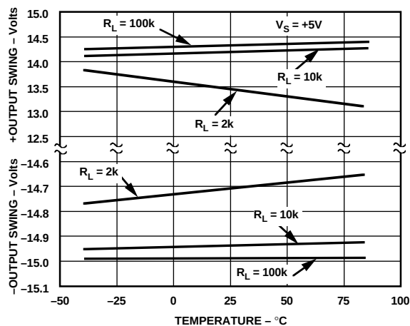
Figure 25. Output Voltage Swing vs. Temperature @ ±15 V
