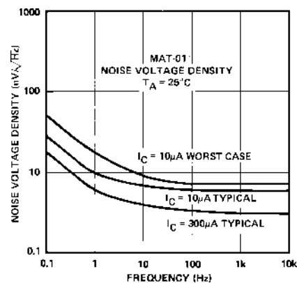
Figure 3. Noise Voltage
