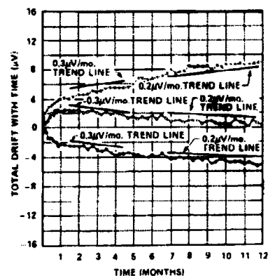
TYPICAL OFFSET VOLTAGE STABILITY vs TIME
