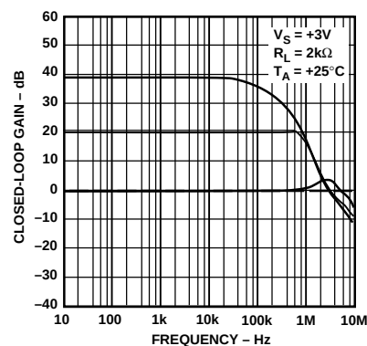
Figure 19. Closed-Loop Gain vs. Frequency (2 kΩ Load)
