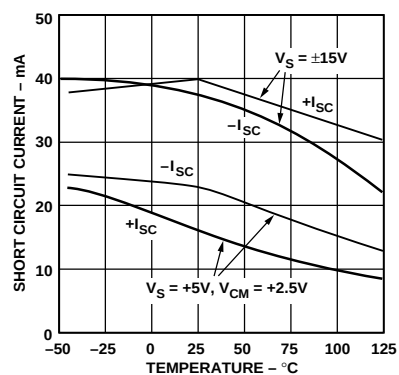
Figure 12. Short Circuit Current vs. Temperature
