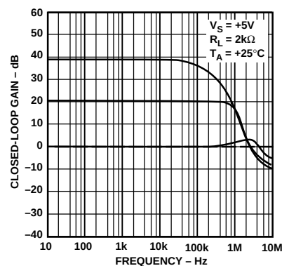
Figure 17. Closed-Loop Gain vs. Frequency (2 kΩ Load)
