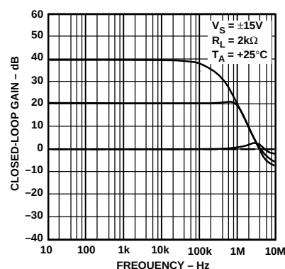
Figure 18. Closed-Loop Gain vs. Frequency (2 kΩ Load)
