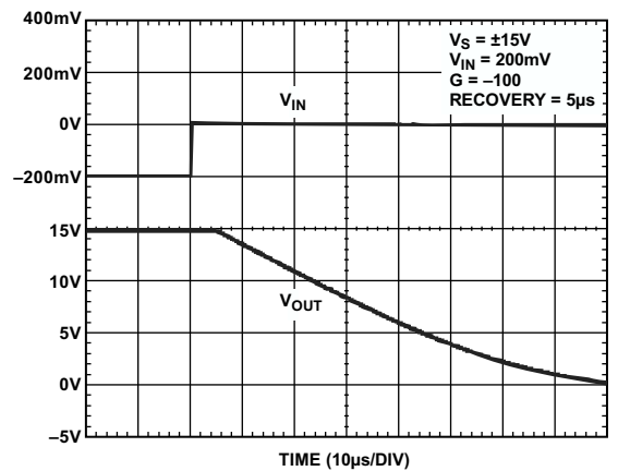
Figure 37. Negative Overload Recovery
