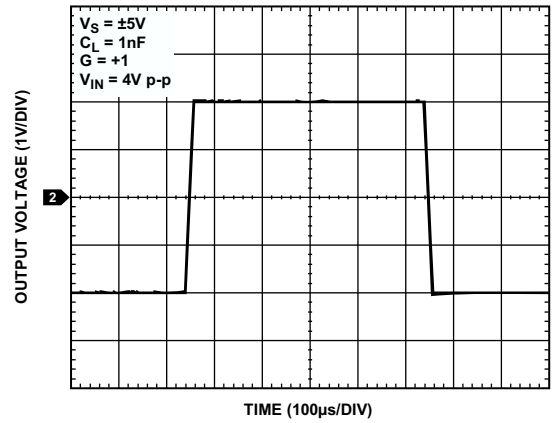
Figure 35. Large-Signal Transient
