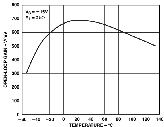
TPC 4. Open-Loop Gain vs. Temperature
