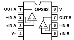
8-Lead TSSOP (RU Suffix)
