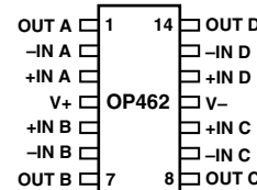
14-Lead Narrow-Body SO (S Suffix)
