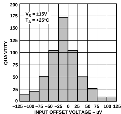
Figure 4. Input Offset Voltage Distribution
