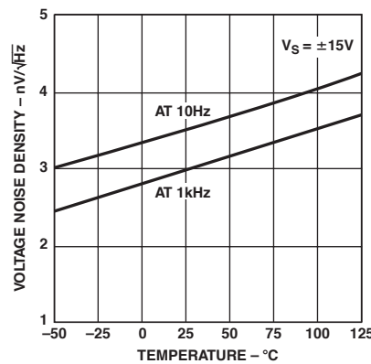
TPC 7. Voltage Noise Density vs. Temperature
