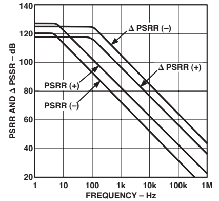
TPC 29. PSRR and ΔPSRR vs. Frequency
