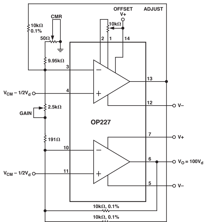
Figure 3. Two Op Amp Instrumentation Amplifier Using OP227 Dual
