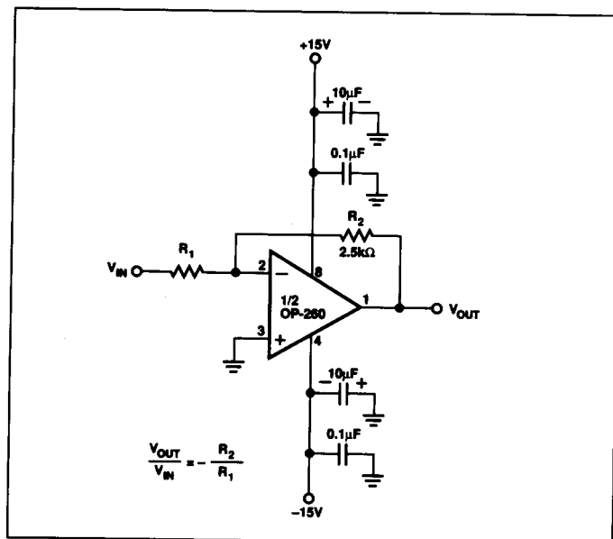
FIGURE 10: The OP-260 as an inverting amplifier.
