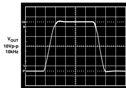
SCALE: VERTICAL-2V/DIV HORIZONTAL-10μs/DIV
