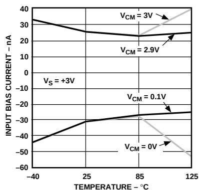
Figure 5. Input Bias Current vs. Temperature, V_S = +3V
