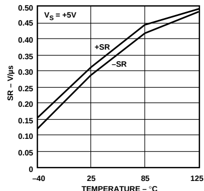
Figure 34. OP491 Slew Rate vs. Temperature, V_S = +5V
