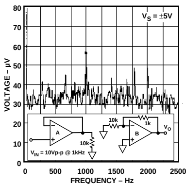
Figure 36. Channel Separation, V_S = \pm 5V
