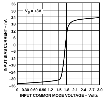
Figure 7. Input Bias Current vs. Common-Mode Voltage, V_S = +3V
