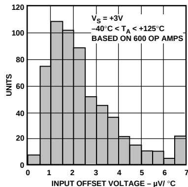
Figure 3. OP291 Input Offset Voltage Drift Distribution, V_S = +3V
