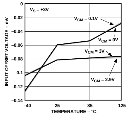
Figure 4. Input Offset Voltage vs. Temperature, V_S = +3V
