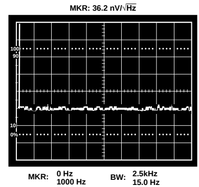
Figure 19. Voltage Noise Density, V_S = +3 V to \pm 5 V , A_{VO} = 1000
