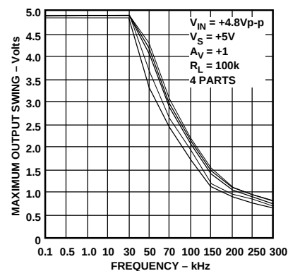
Figure 37. Maximum Output Swing vs. Frequency, V_S = +5V
