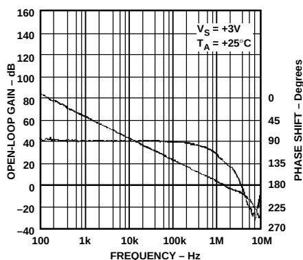
Figure 9. Open-Loop Gain & Phase vs. Frequency, V_S = +3V
