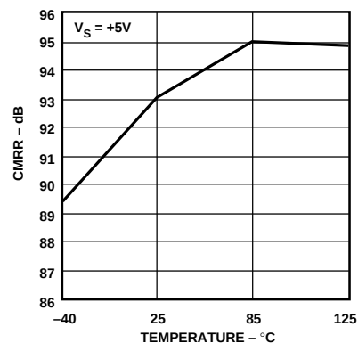
Figure 31. CMRR vs. Temperature, V_S = +5V
