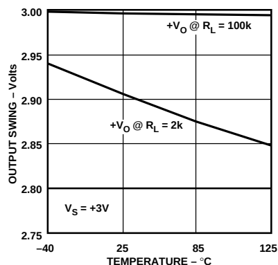
Figure 8. Output Voltage Swing vs. Temperature, V_S = +3V
