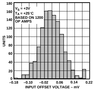
Figure 2. OP291 Input Offset Voltage Distribution, V_S = +3V
