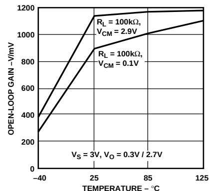
Figure 10. Open-Loop Gain vs. Temperature, V_S = +3V
