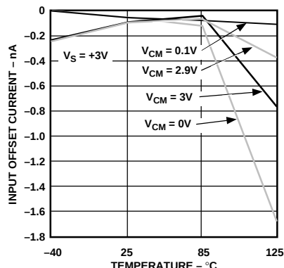
Figure 6. Input Offset Current vs. Temperature, V_S = +3V
