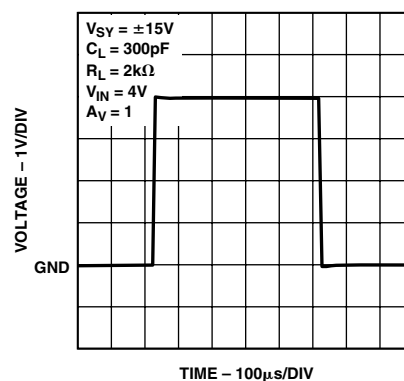
TPC 9. Large Signal Transient Response
