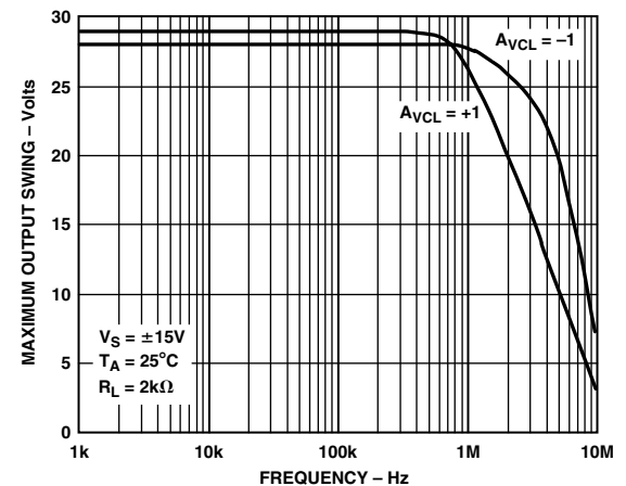
TPC 6. Max V_{OUT} Swing vs. Frequency
