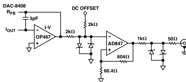
Figure 15. DAC V_{OUT} Settling Time Circuit
