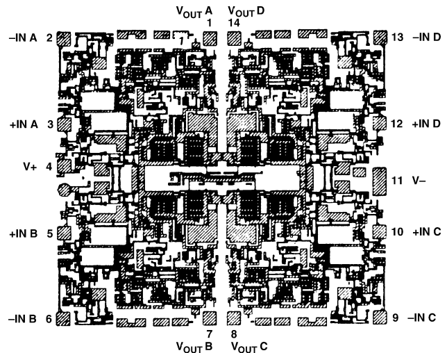
OP467 Die Size 0.111 \times 0.100 inch, 11,100 sq. mils Substrate is Connected to V+, Number of Transistors 165
