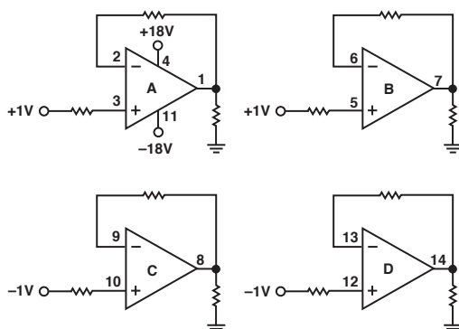
Figure 3. Burn-In Circuit
