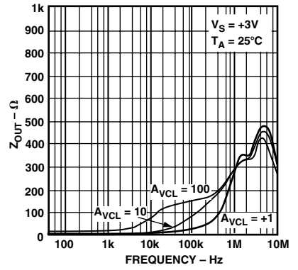
TPC 51. Output Impedance vs. Frequency
