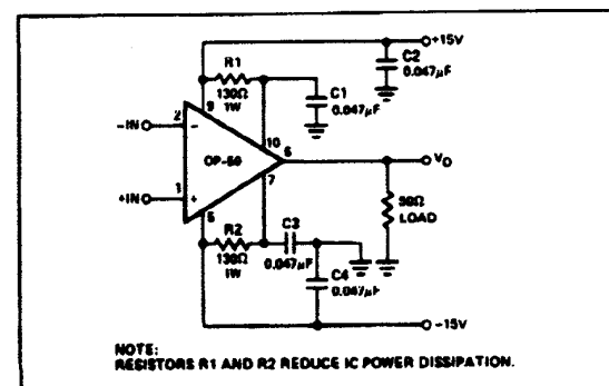
FIGURE 5: DRIVING 50\Omega LOADS
