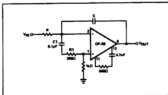
FIGURE 3: INTEGRATOR
