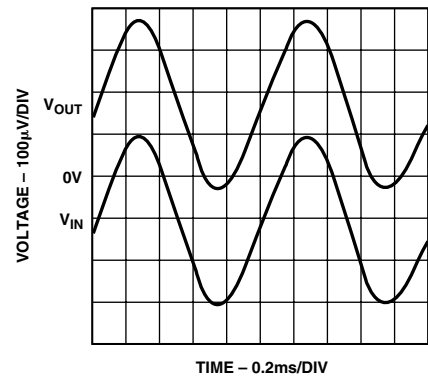
Figure 1. Input and Output Signals with V_{CM} < 0\text{ V}
