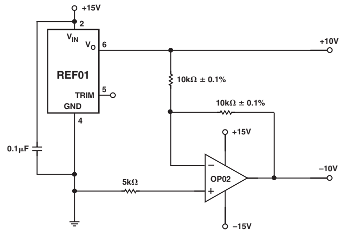
Figure 8. ±10 V Reference
