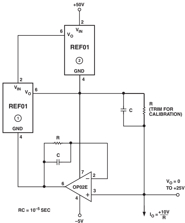
Figure 10. Precision Current Source
