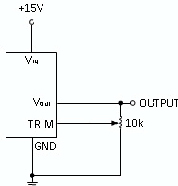
Vout Trim Circuit
