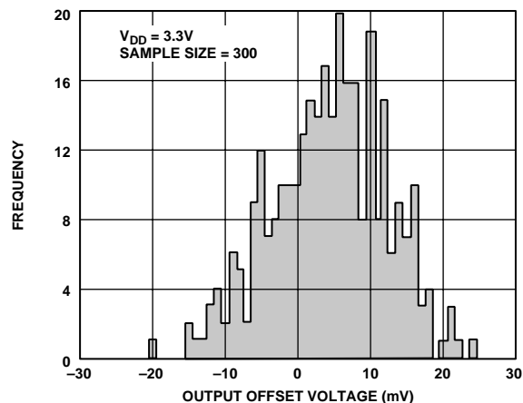
Figure 37. Output Offset Voltage Distribution
