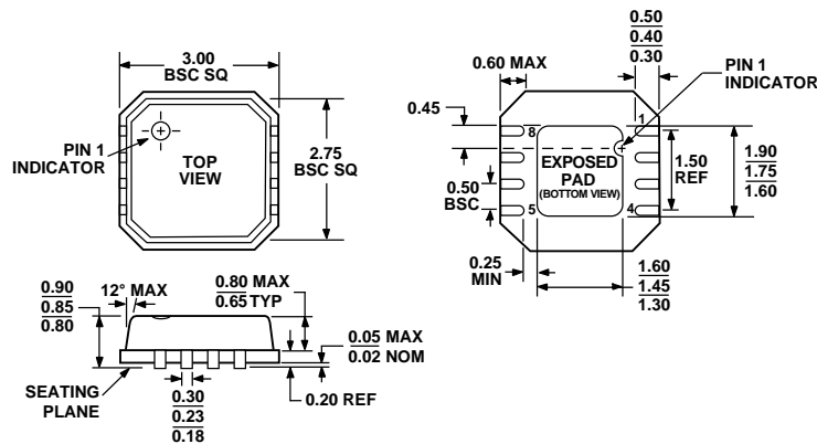
Figure 53. 8-Lead Frame Chip Scale Package [LFCSF] 3 mm × 3 mm Body (CP-8-2) Dimensions shown in millimeters
