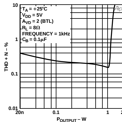
Figure 8. THD+N vs. P_{OUT}
