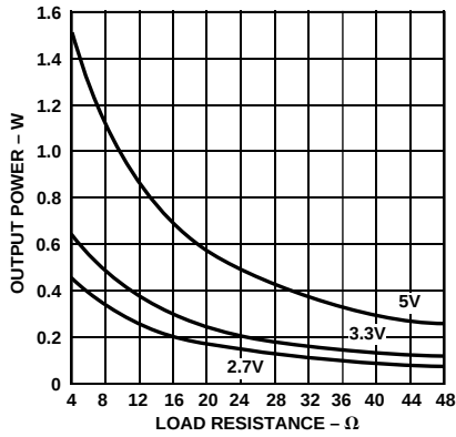
Figure 31. P_{OUT} vs. Load Resistance
