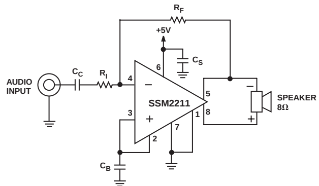
Figure 39. A Typical Configuration
