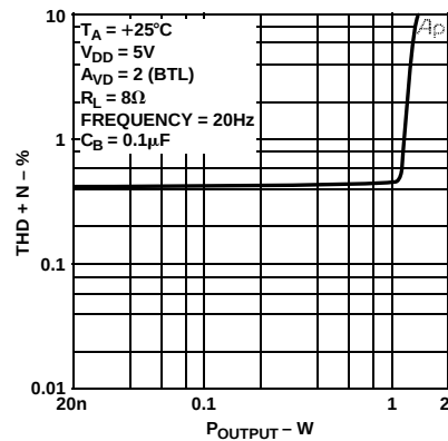
Figure 7. THD+N vs. P_{OUT}
