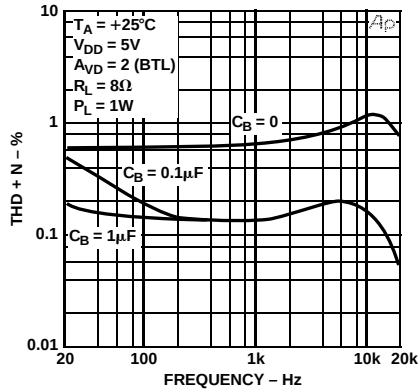
Figure 4. THD+N vs. Frequency
