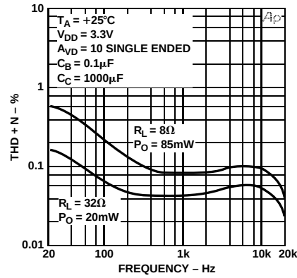
Figure 23. THD+N vs. Frequency
