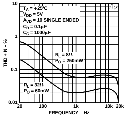
Figure 22. THD+N vs. Frequency
