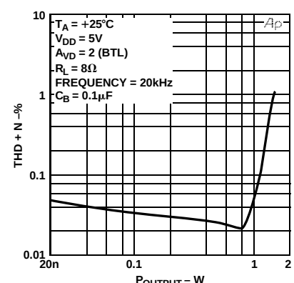
Figure 9. THD+N vs. P_{OUT}
