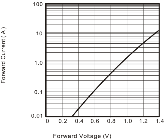
Fig.2 - Forward Characteristics
